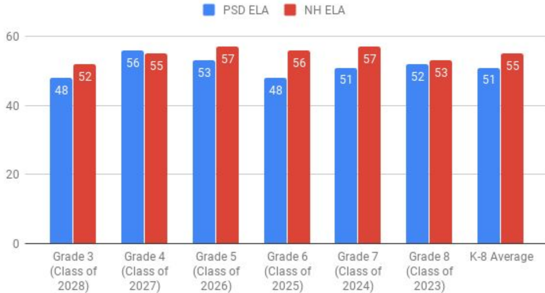
PSD ELA and NH ELA 2019
