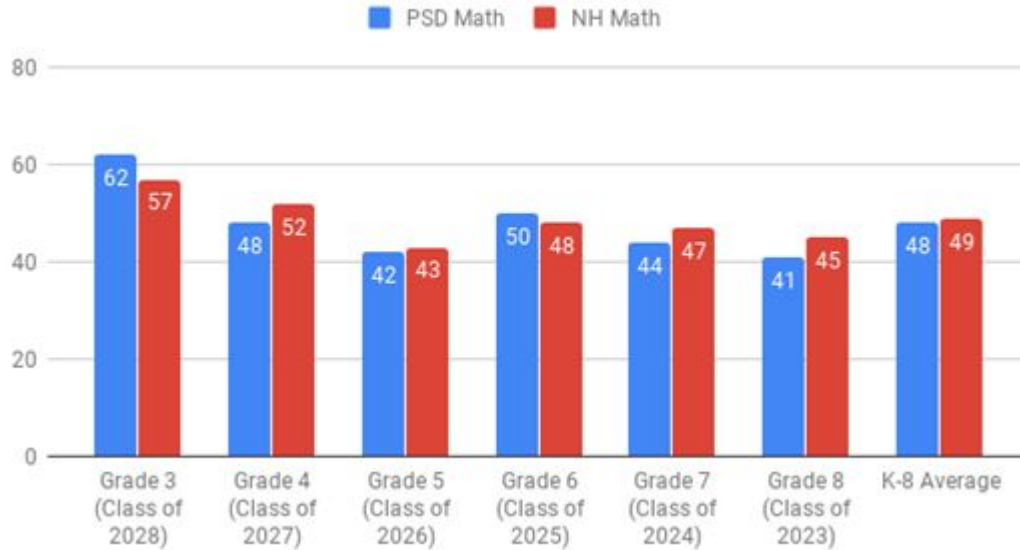
PSD Math and NH Math 2019
